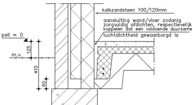
kalkzandsteendetail 5
