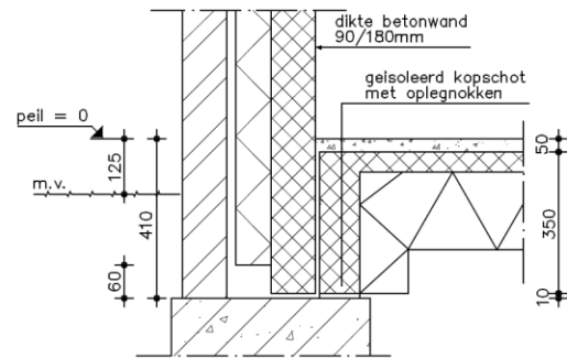
beton/giet detail 1B/G
